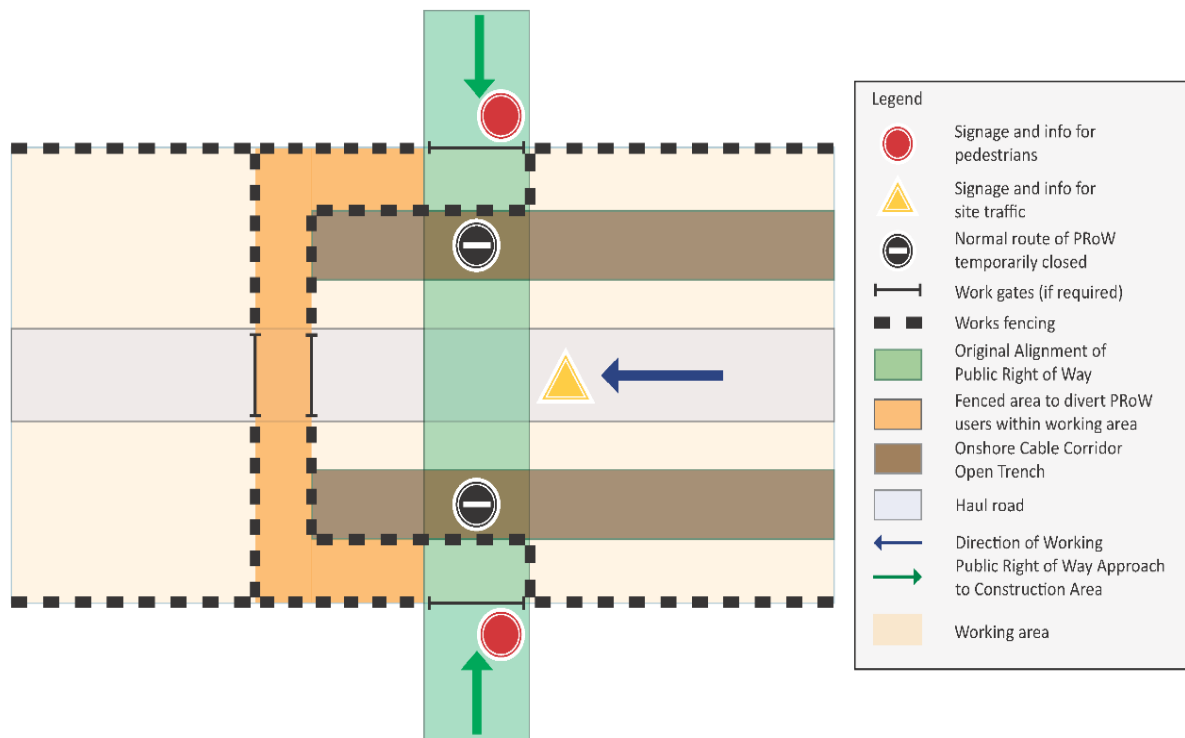
Figure 1.3: Illustrative diagram of temporary diversion of a PRow
